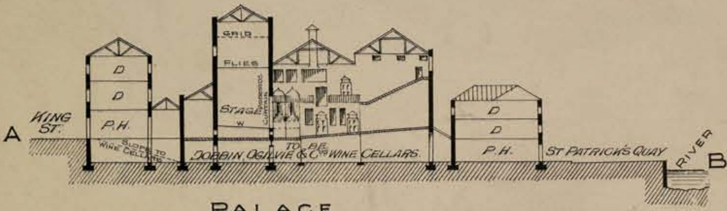
PALACE THEATRE OF VARIETIES SECTION ON LINE A-B.
